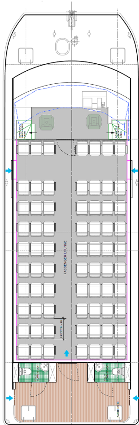
DECK PLAN
